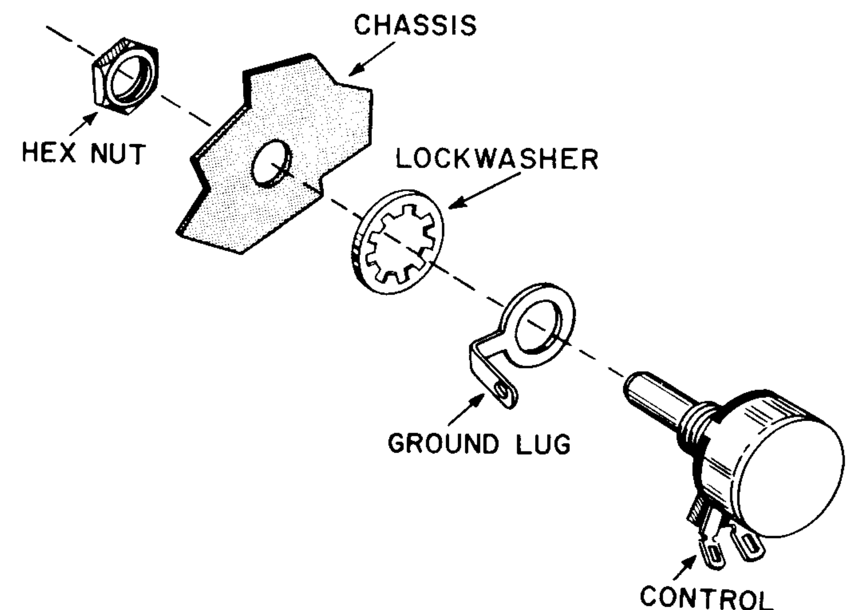
FIGURE 5. HOW TO MOUNT A CONTROL USING A GROUND LUG
