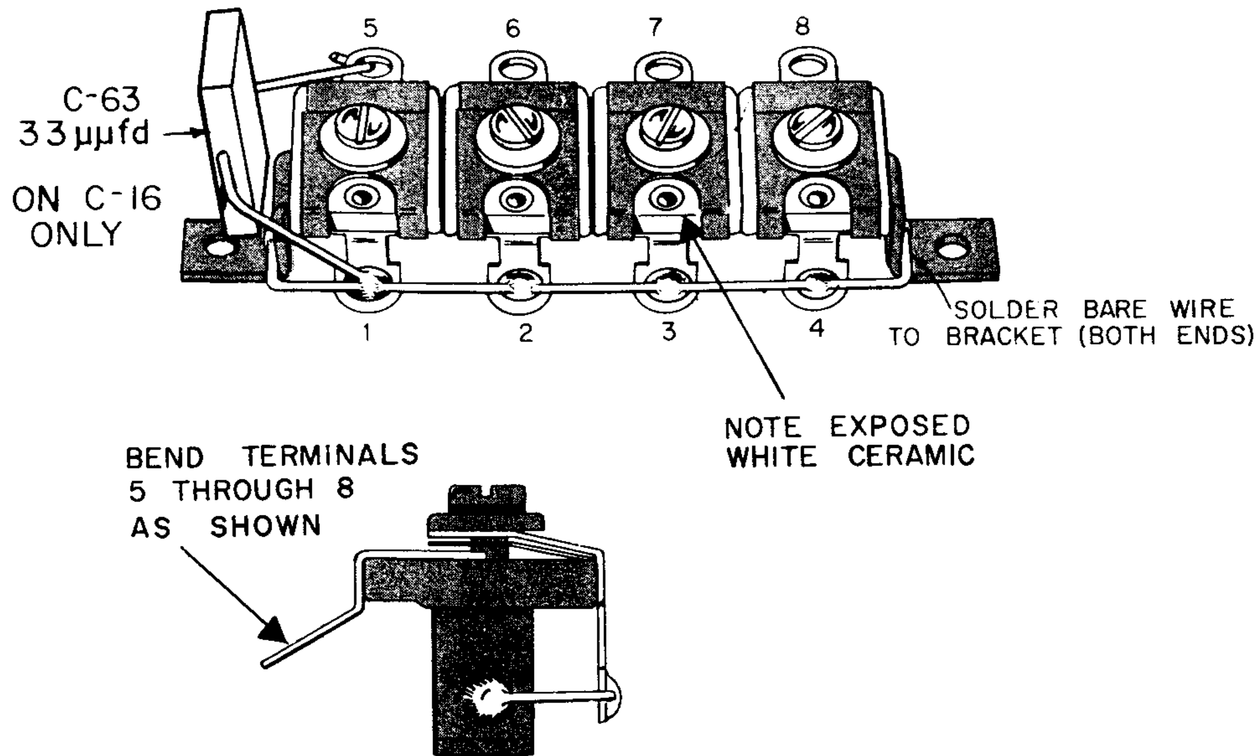
FIGURE 14. PREPARING THE TRIMMER STRIPS
