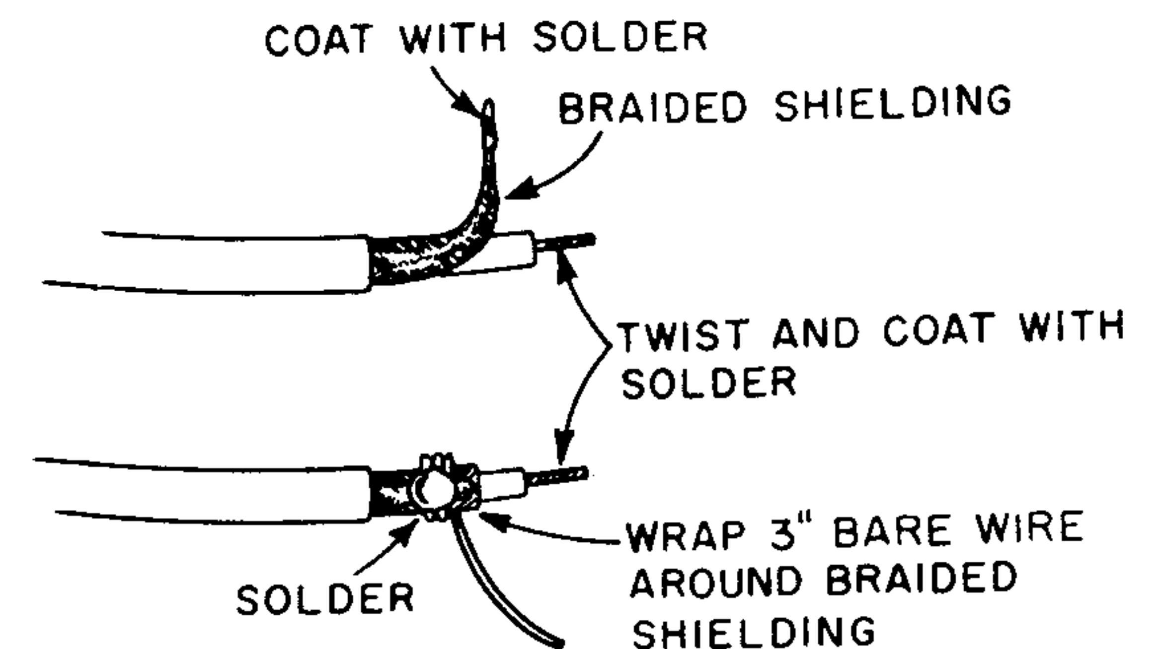
FIGURE 9. PREPARING INSULATED SHIELDED WIRES
