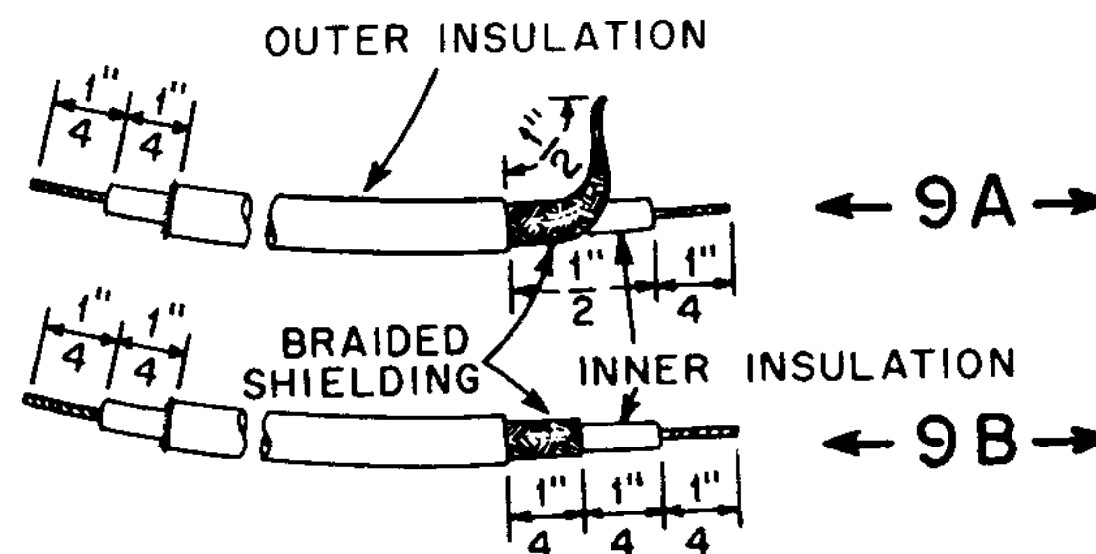
FIGURE 9. PREPARING INSULATED SHIELDED WIRES
