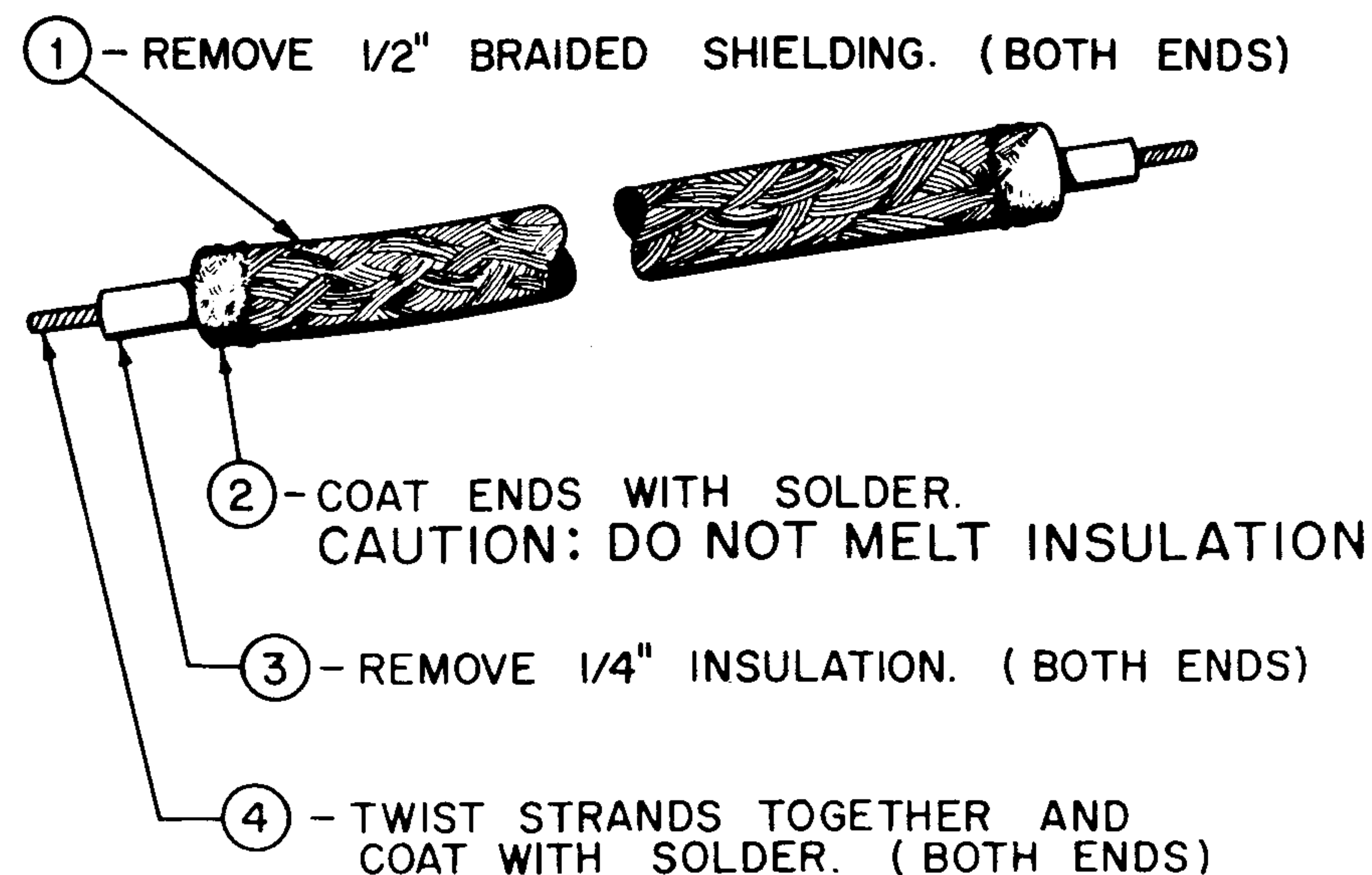
FIGURE 7. PREPARING UNINSULATED SHIELDED WIRES
