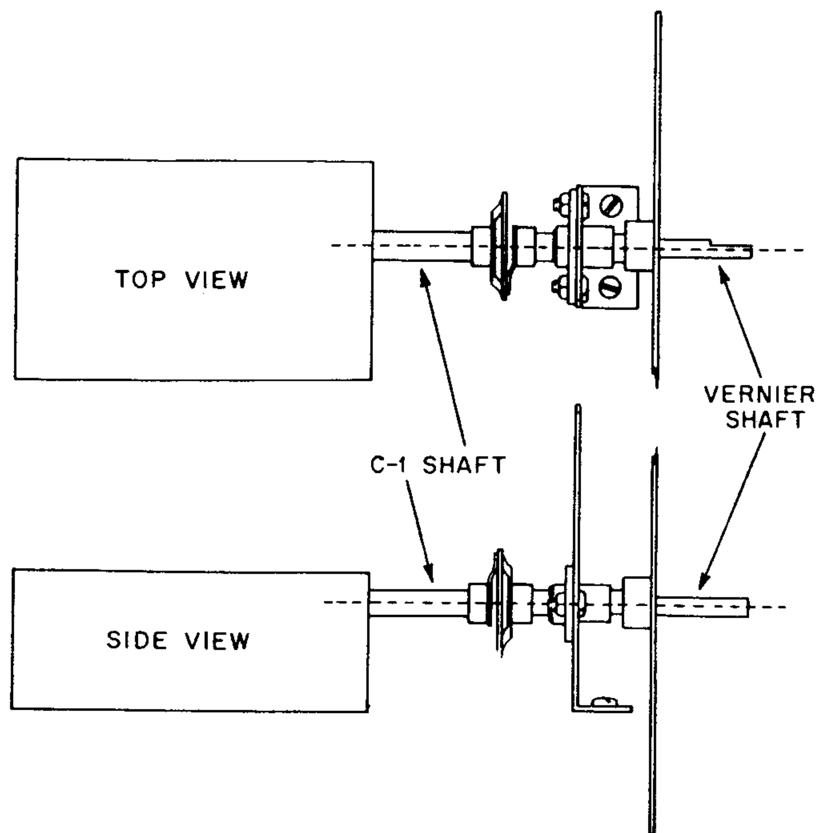
FIGURE 20A. SHAFT ALIGNMENT
